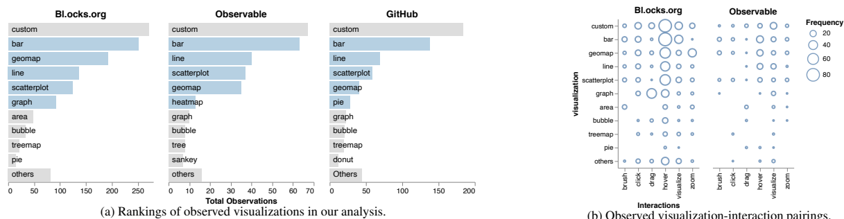
Figure 2: Results from analysis carried out on the three example corpus (a) presents the frequency of the top visualization types and their corresponding interactions observed in our datasets. Visualizations with 1% and less frequency are captured in the “others” category. (b) shows the number of times different interaction types were implemented for each visualization type in our corpus
