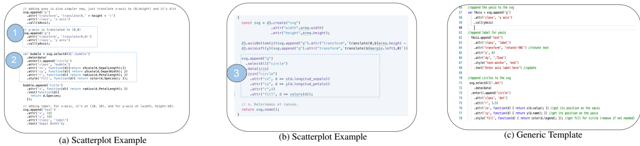
Figure 3: Reoccurring code blocks (1, 2 & 3) in two scatterplot examples (A & B) are synthesized into a generic scatterplots template (C).
